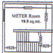
METER ROOM PLAN
